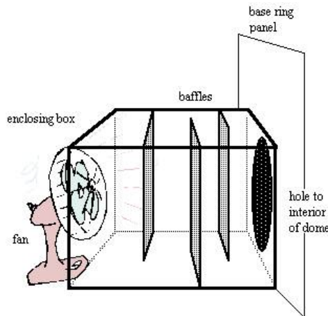
Figure 11. A ventilation system for your dome.
